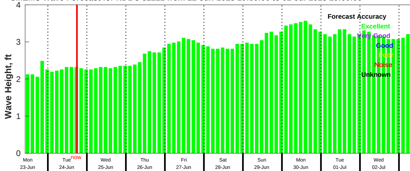
CMEMS Wave Forecast for NDBC 52211 from 22-Jun-2025 10:00:00 to 02-Jul-2025 10:00:00
