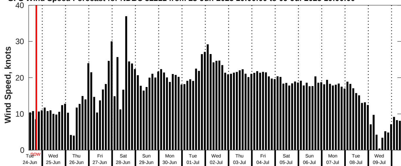
GFS Wind Speed Forecast for NDBC 52211 from 23-Jun-2025 10:00:00 to 09-Jul-2025 10:00:00
