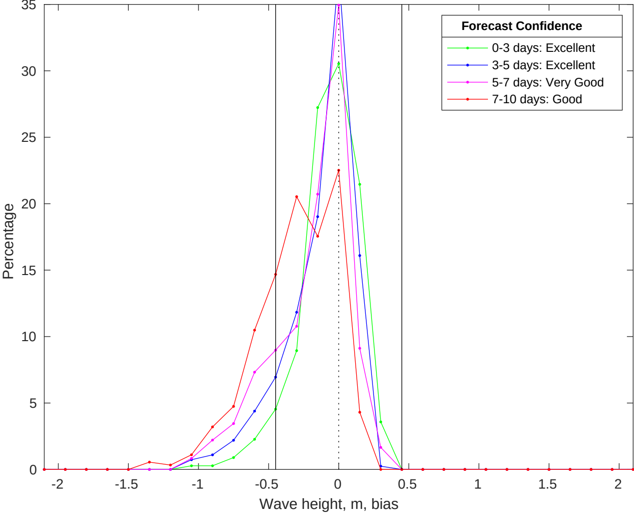
NDBC 52212 vs CMEMS Waves Bias Histogram: 23-Jun-2025
