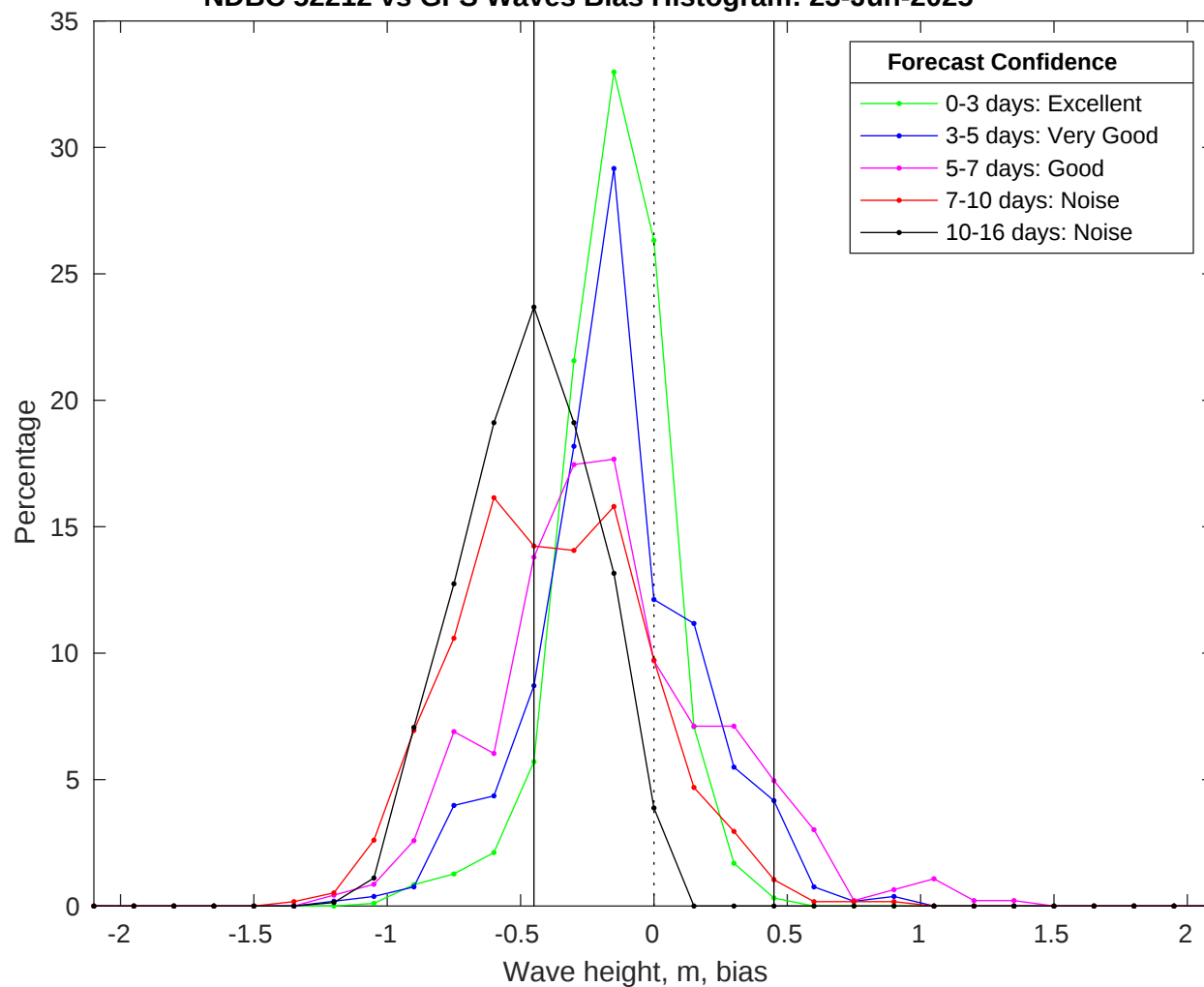
NDBC 52212 vs GFS Waves Bias Histogram: 23-Jun-2025
