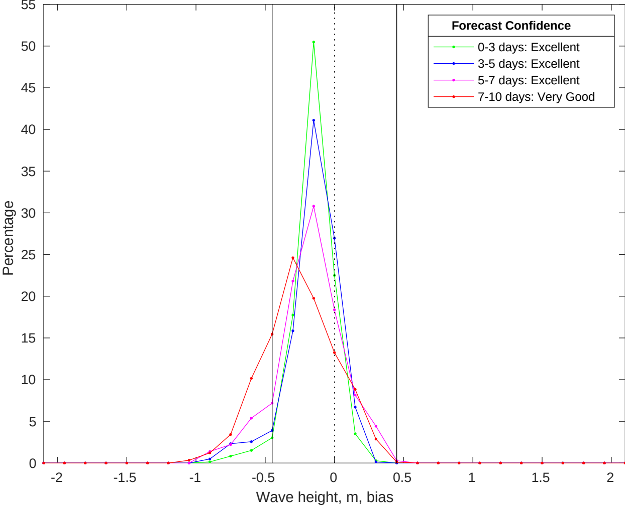
NDBC 52213 vs CMEMS Waves Bias Histogram: 23-Jun-2025
