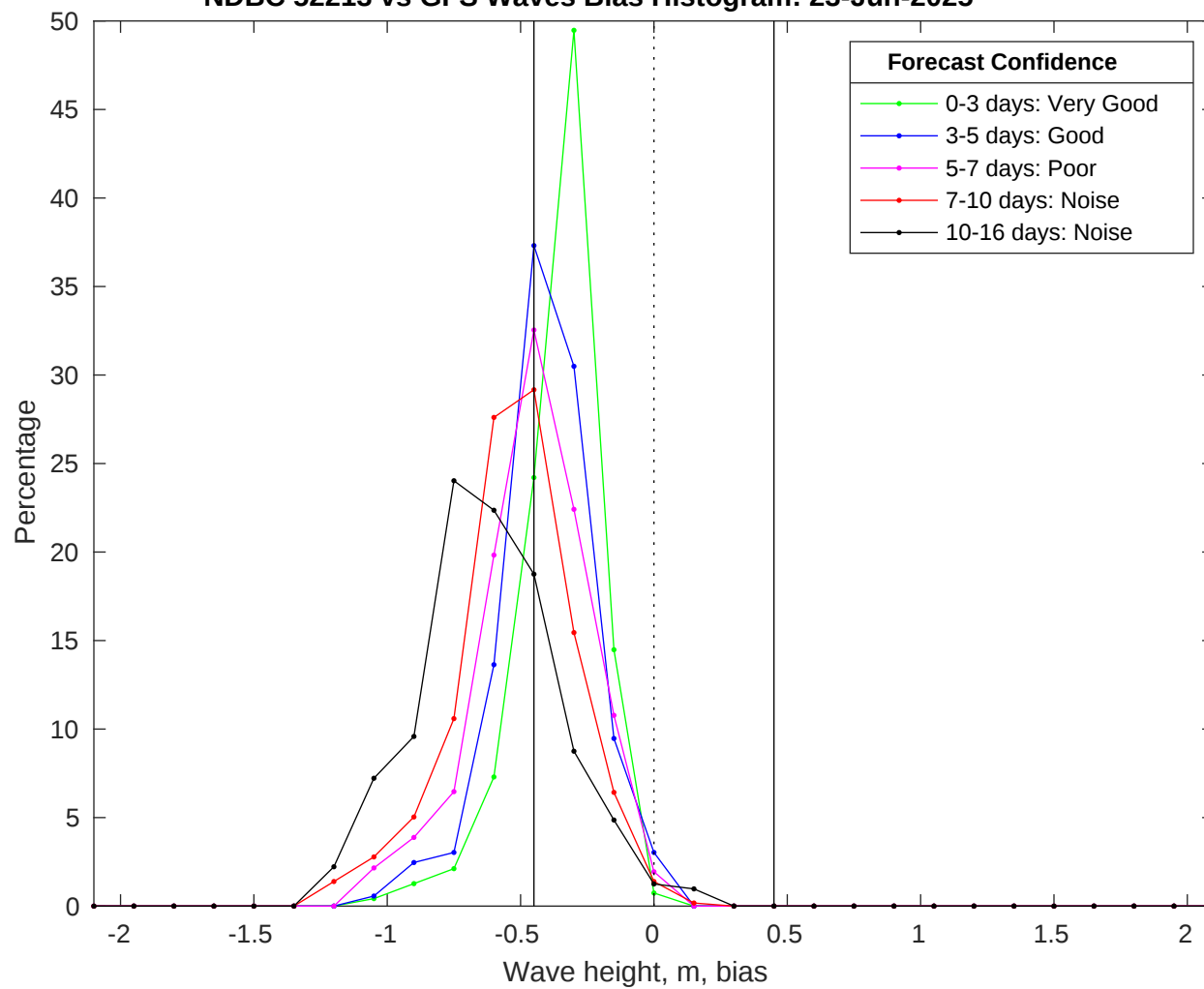
NDBC 52213 vs GFS Waves Bias Histogram: 23-Jun-2025
