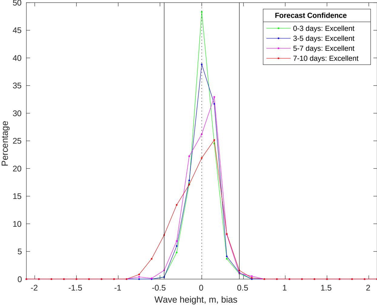
NDBC 41004 vs CMEMS Waves Bias Histogram: 24-Jun-2025
