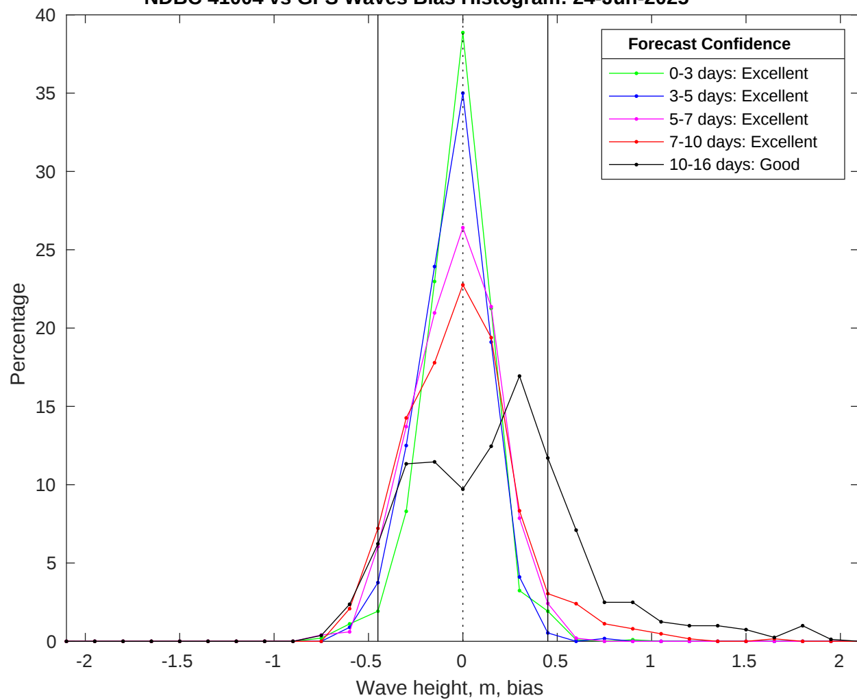
NDBC 41004 vs GFS Waves Bias Histogram: 24-Jun-2025
