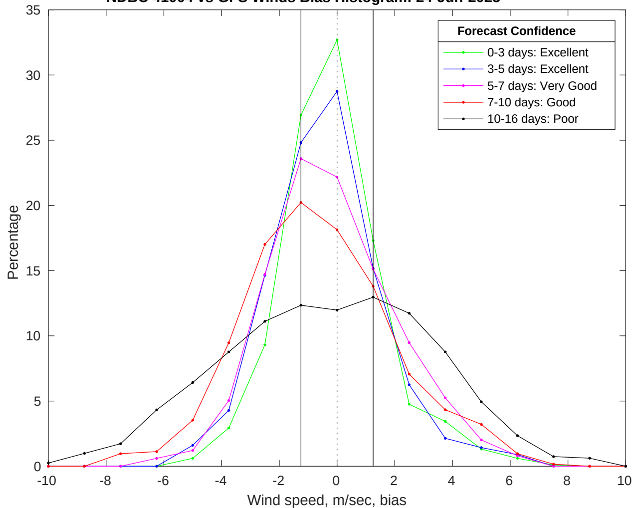
NDBC 41004 vs GFS Winds Bias Histogram: 24-Jun-2025
