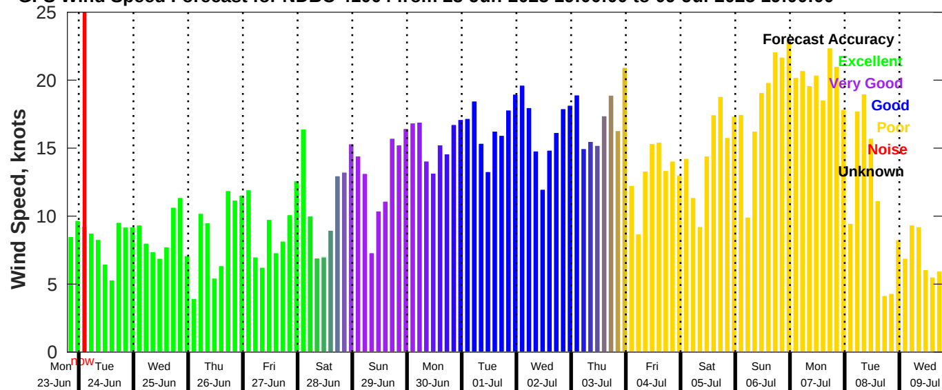
GFS Wind Speed Forecast for NDBC 41004 from 23-Jun-2025 19:00:00 to 09-Jul-2025 19:00:00
