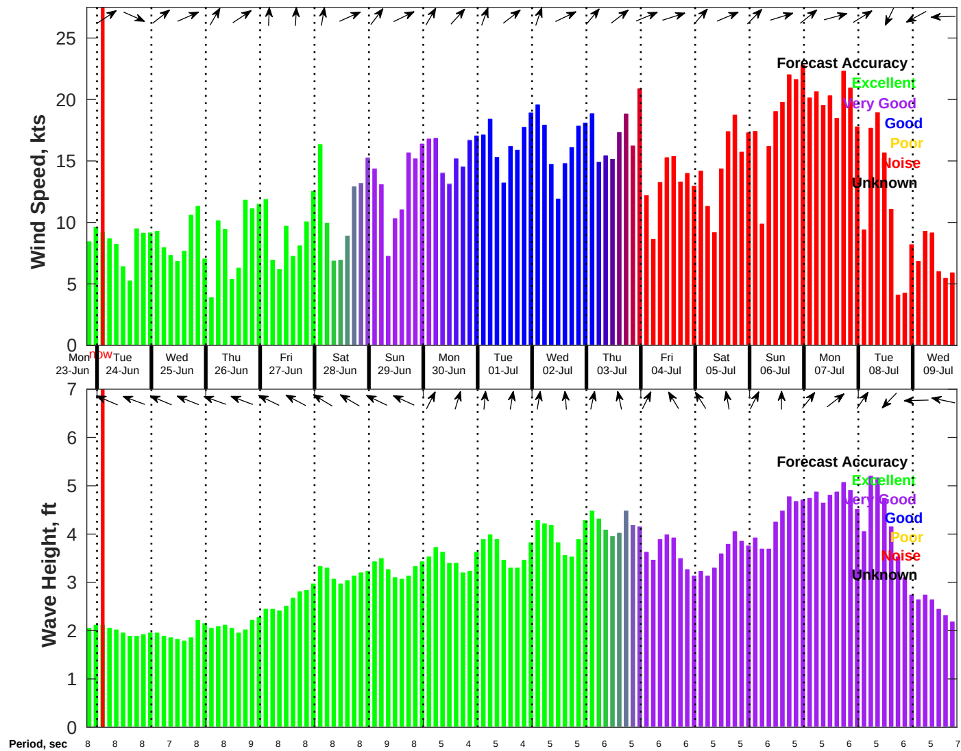
Wind & Wave Forecast for NDBC 41004 from 23-Jun-2025 19:00:00 to 09-Jul-2025 19:00:00
