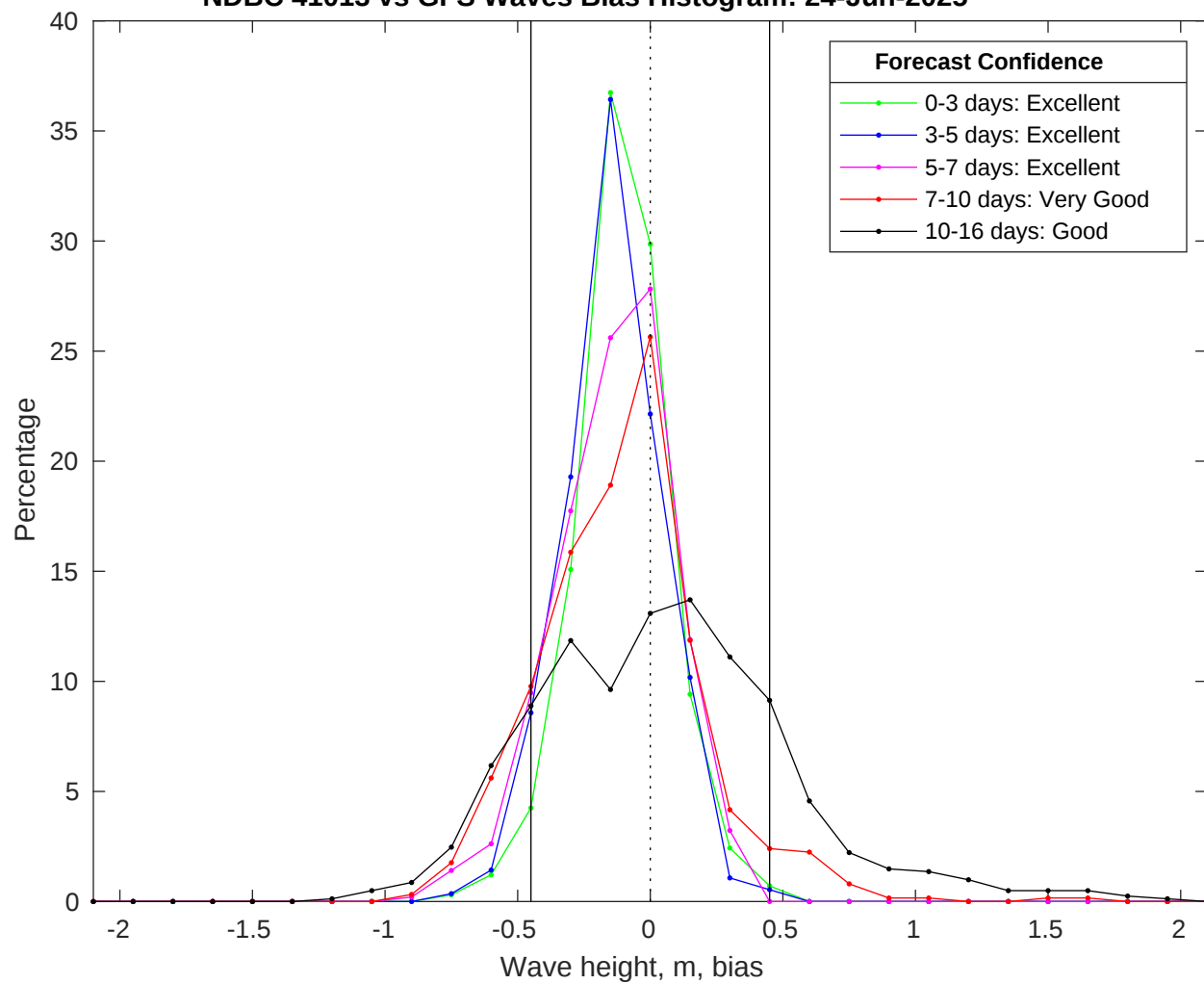
NDBC 41013 vs GFS Waves Bias Histogram: 24-Jun-2025
