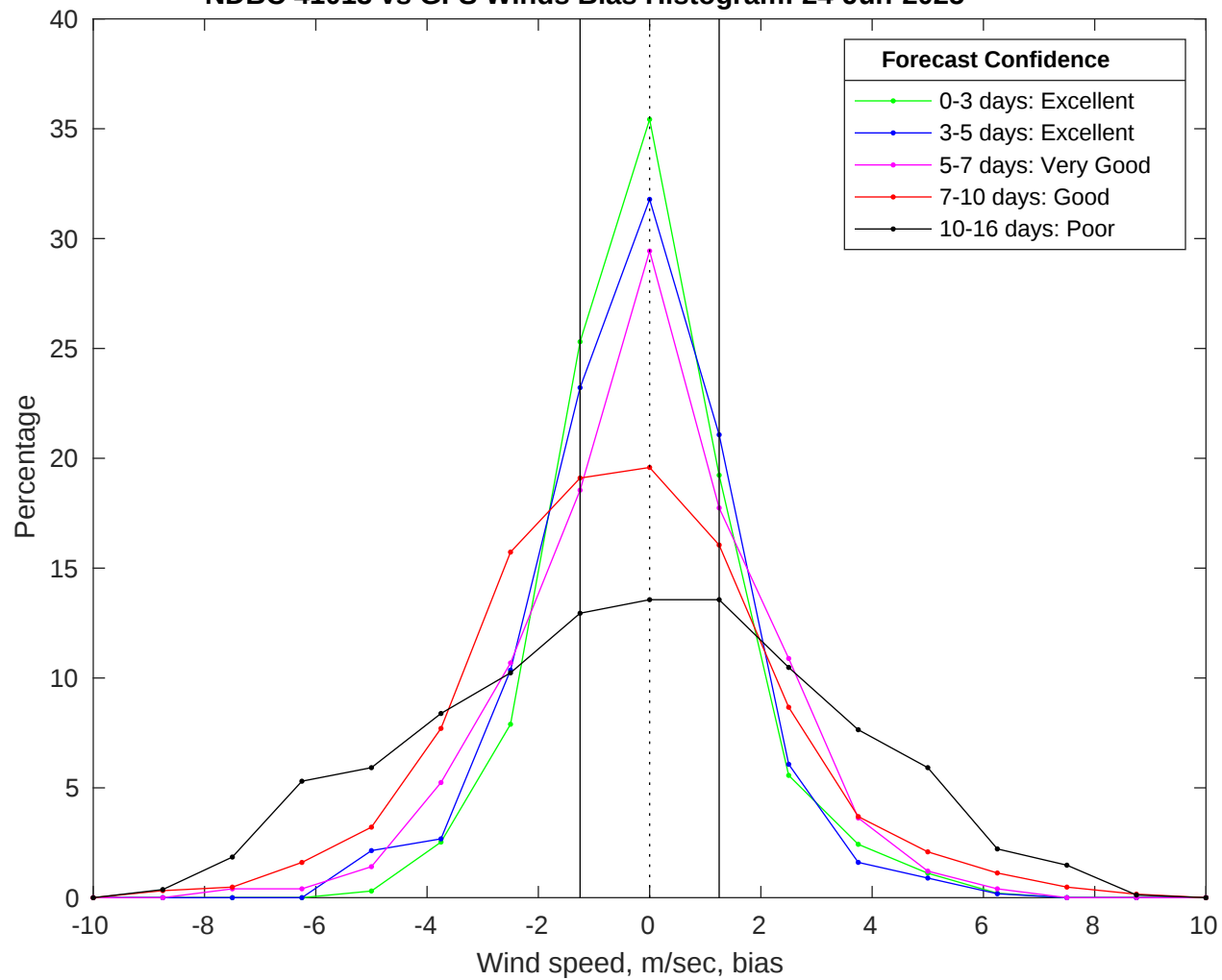
NDBC 41013 vs GFS Winds Bias Histogram: 24-Jun-2025
