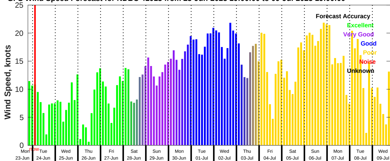
GFS Wind Speed Forecast for NDBC 41013 from 23-Jun-2025 19:00:00 to 09-Jul-2025 19:00:00
