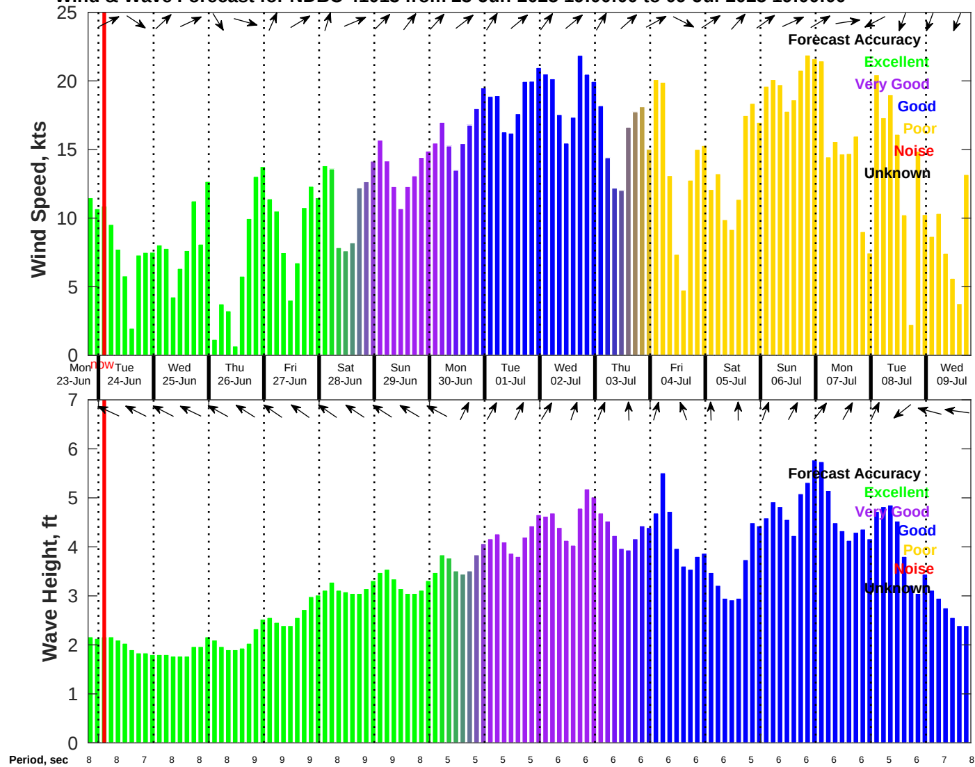
Wind & Wave Forecast for NDBC 41013 from 23-Jun-2025 19:00:00 to 09-Jul-2025 19:00:00
