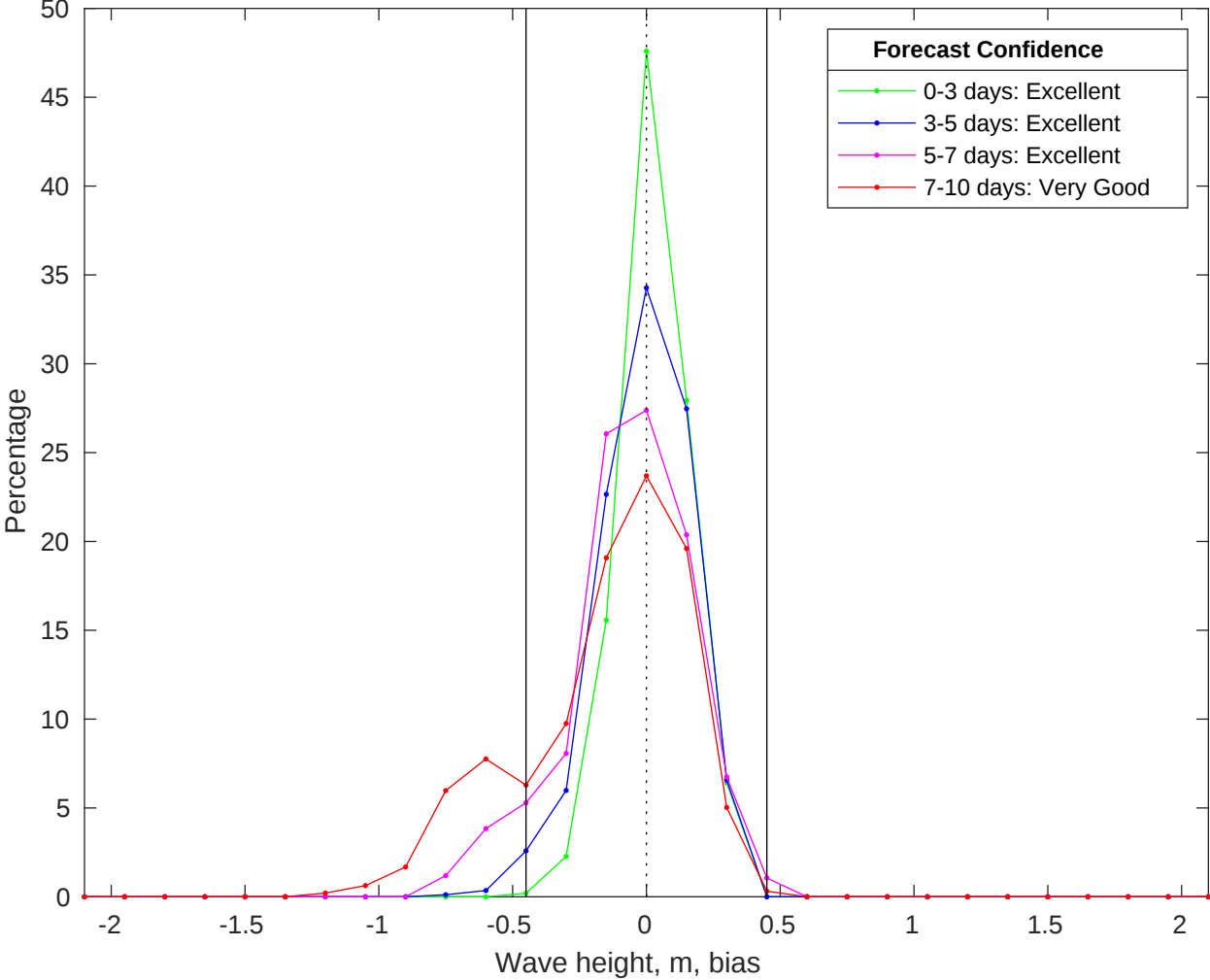
NDBC 41040 vs CMEMS Waves Bias Histogram: 24-Jun-2025
