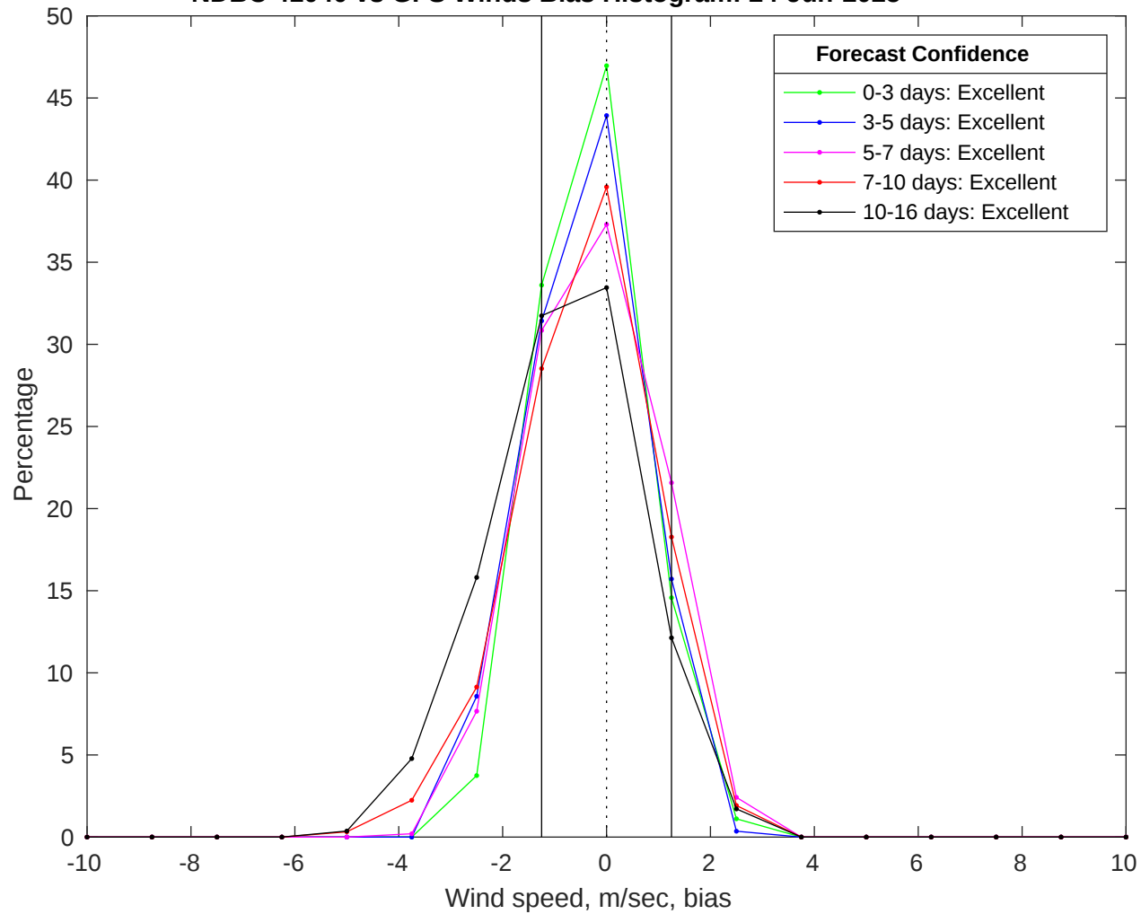
NDBC 41040 vs GFS Winds Bias Histogram: 24-Jun-2025
