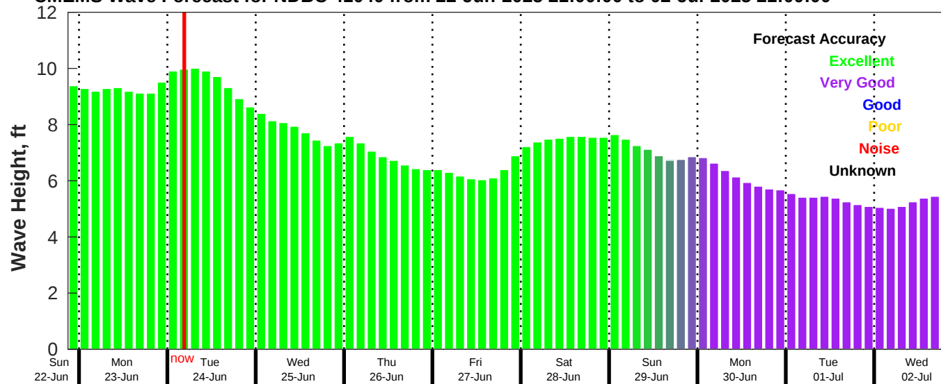
CMEMS Wave Forecast for NDBC 41040 from 22-Jun-2025 21:00:00 to 02-Jul-2025 21:00:00
