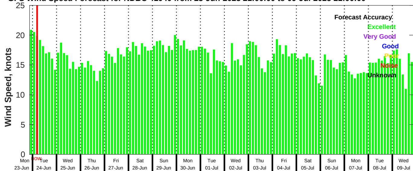
GFS Wind Speed Forecast for NDBC 41040 from 23-Jun-2025 21:00:00 to 09-Jul-2025 21:00:00
