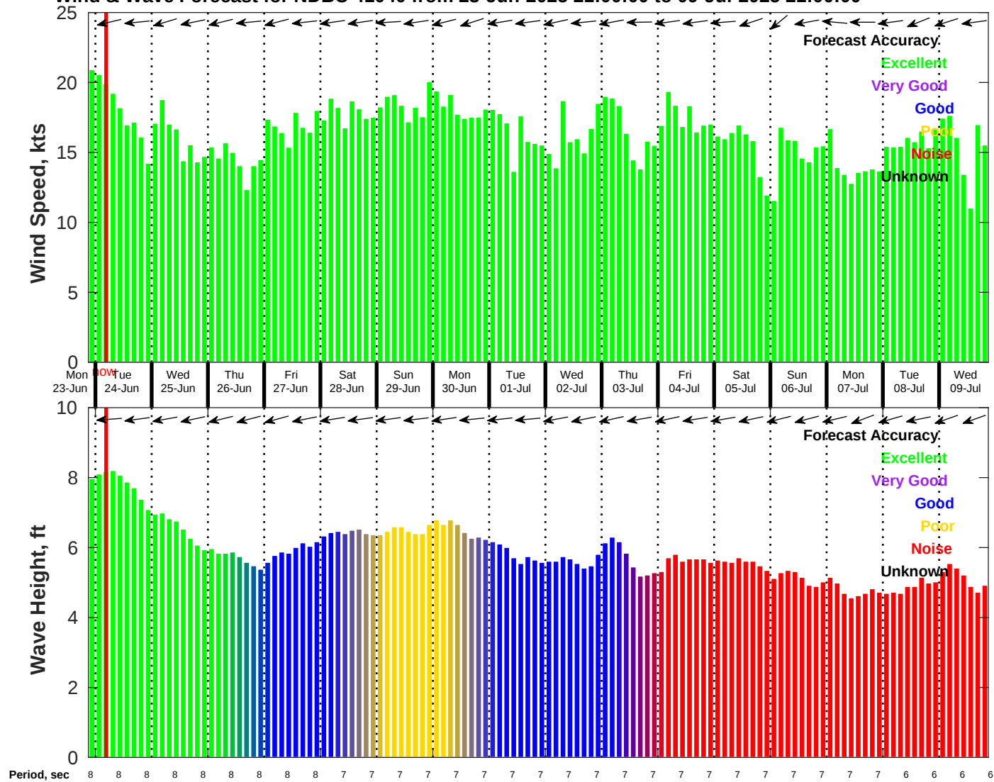
Wind & Wave Forecast for NDBC 41040 from 23-Jun-2025 21:00:00 to 09-Jul-2025 21:00:00
