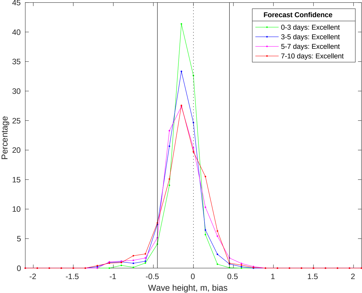
NDBC 42019 vs CMEMS Waves Bias Histogram: 24-Jun-2025
