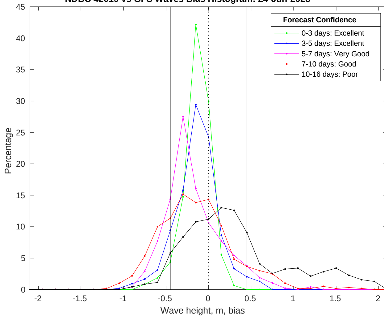
NDBC 42019 vs GFS Waves Bias Histogram: 24-Jun-2025
