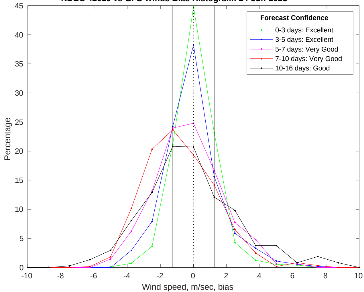
NDBC 42019 vs GFS Winds Bias Histogram: 24-Jun-2025
