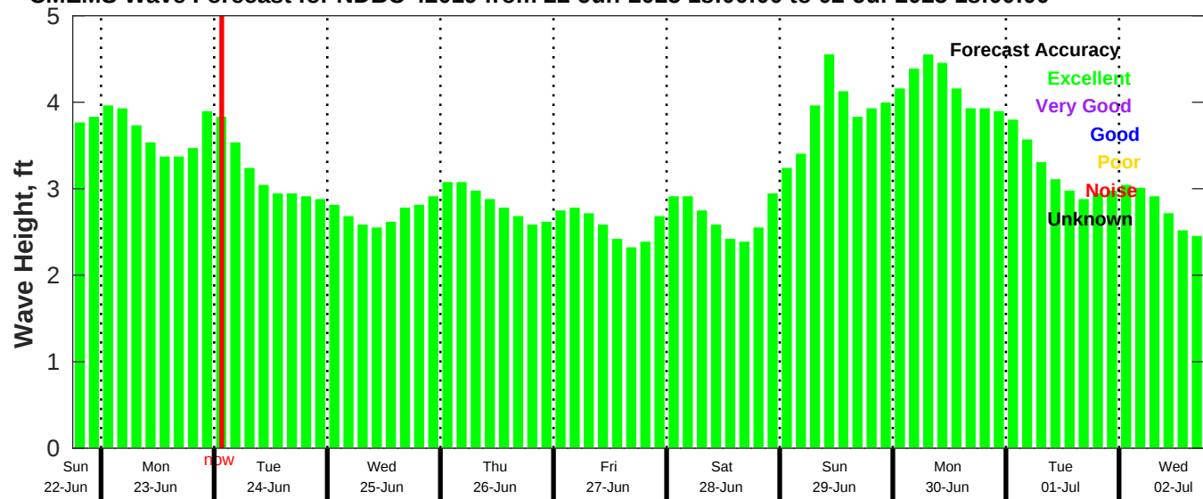
CMEMS Wave Forecast for NDBC 42019 from 22-Jun-2025 18:00:00 to 02-Jul-2025 18:00:00
