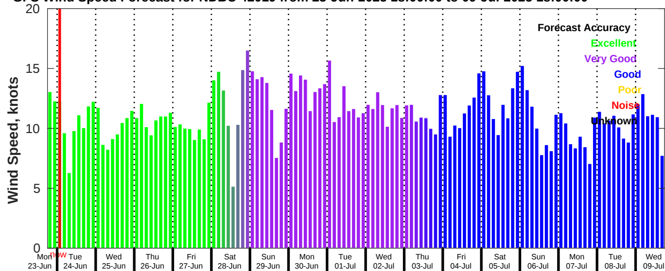
GFS Wind Speed Forecast for NDBC 42019 from 23-Jun-2025 18:00:00 to 09-Jul-2025 18:00:00
