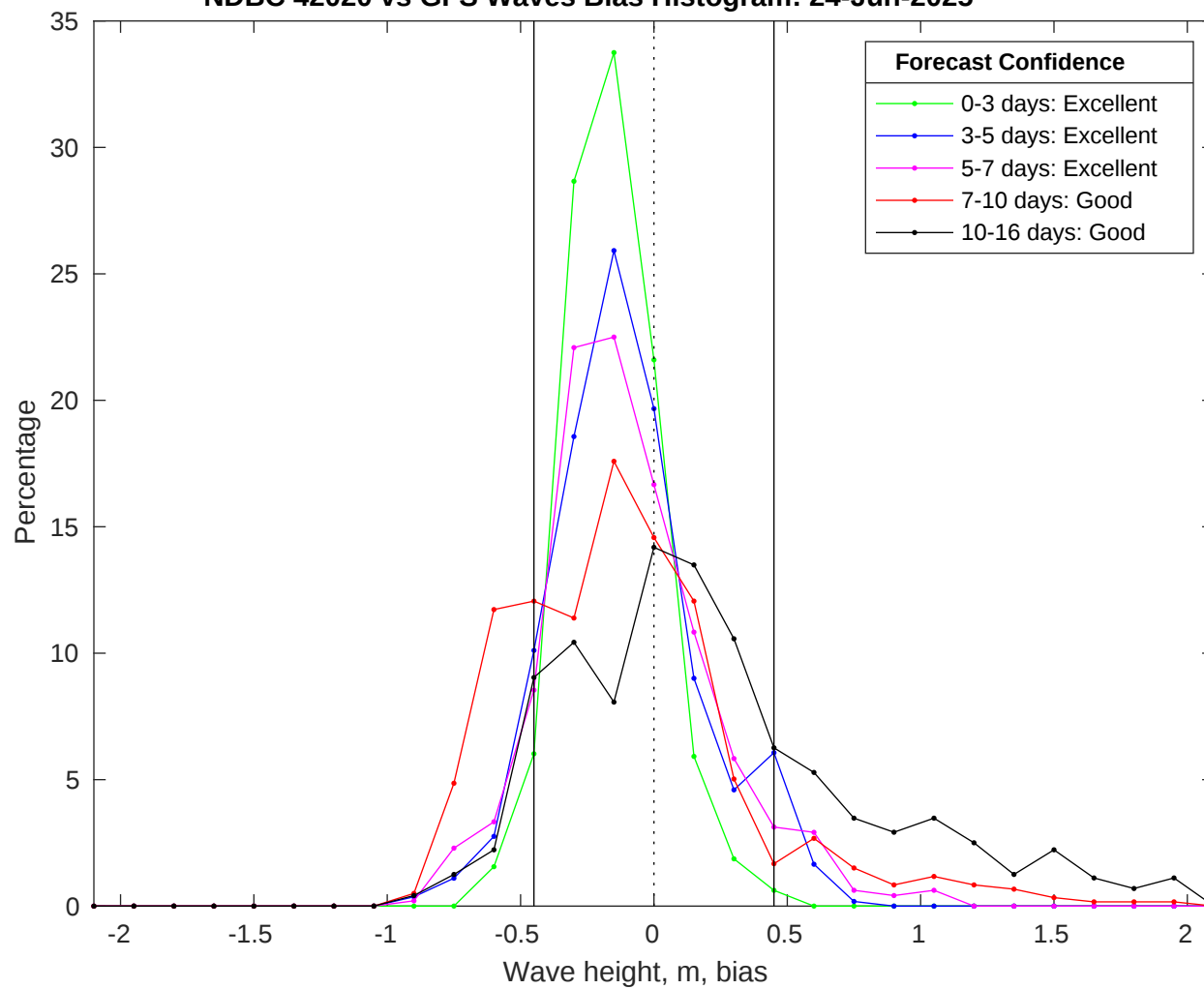
NDBC 42020 vs GFS Waves Bias Histogram: 24-Jun-2025
