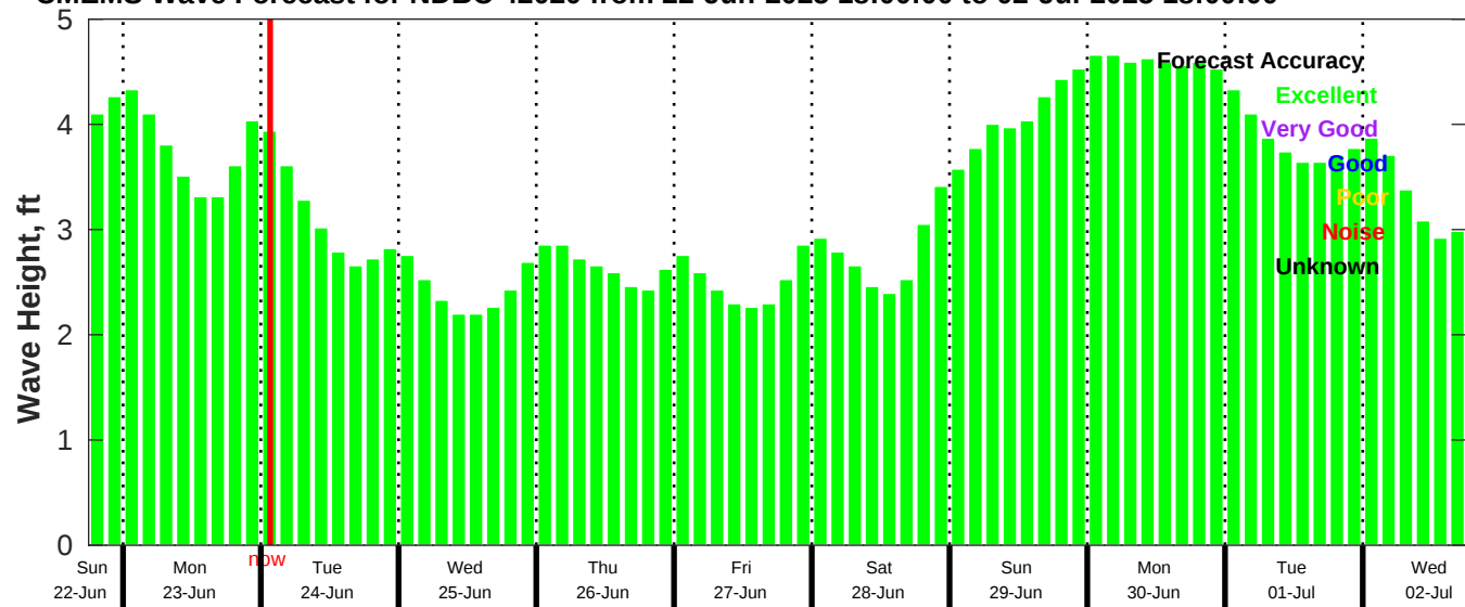
CMEMS Wave Forecast for NDBC 42020 from 22-Jun-2025 18:00:00 to 02-Jul-2025 18:00:00
