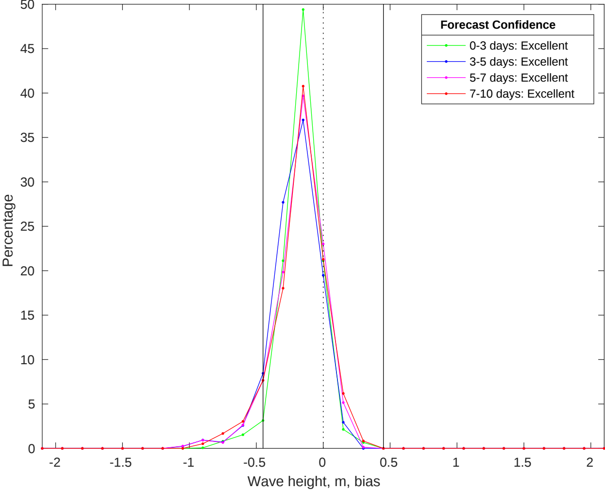
NDBC 42035 vs CMEMS Waves Bias Histogram: 24-Jun-2025
