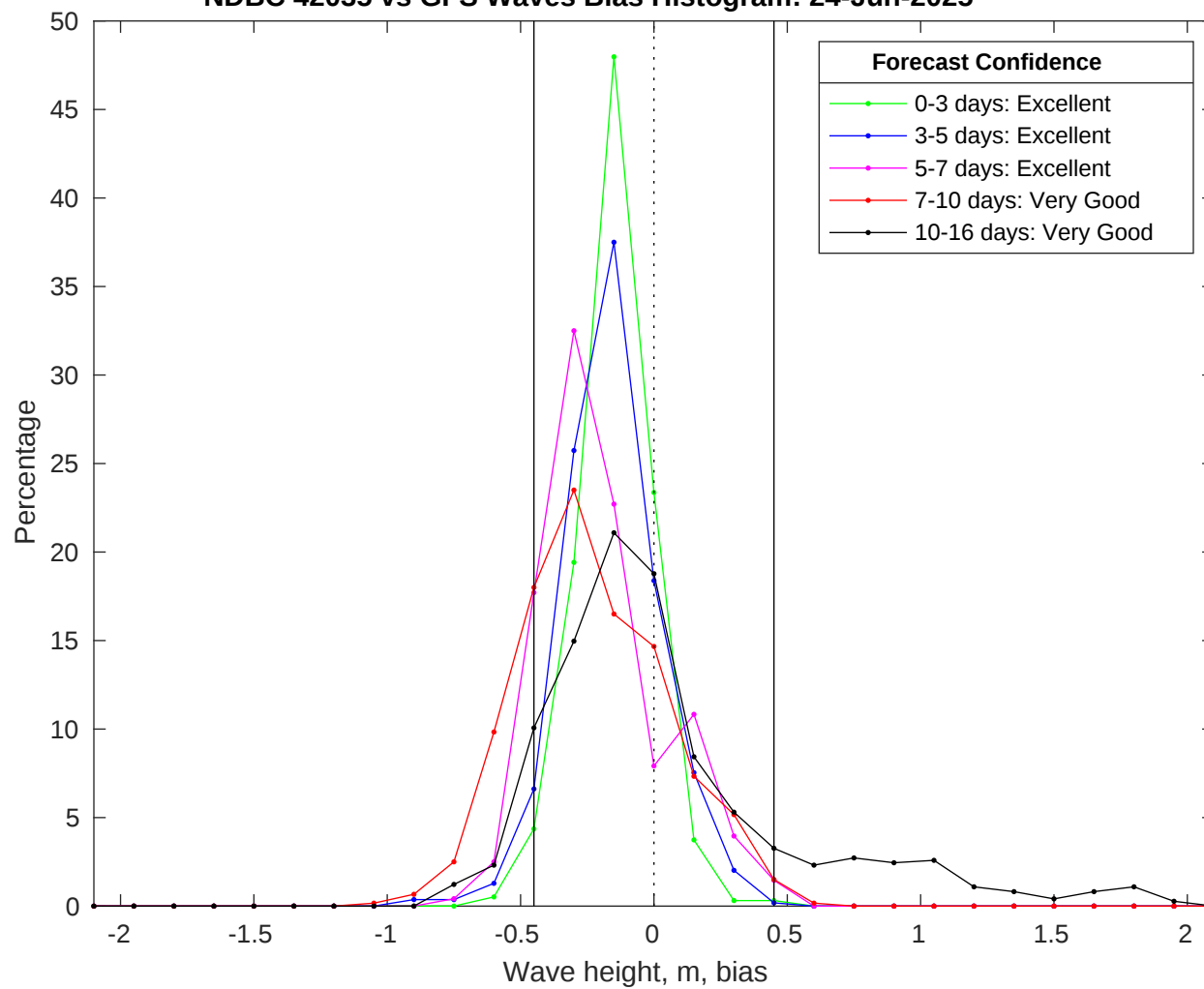
NDBC 42035 vs GFS Waves Bias Histogram: 24-Jun-2025
