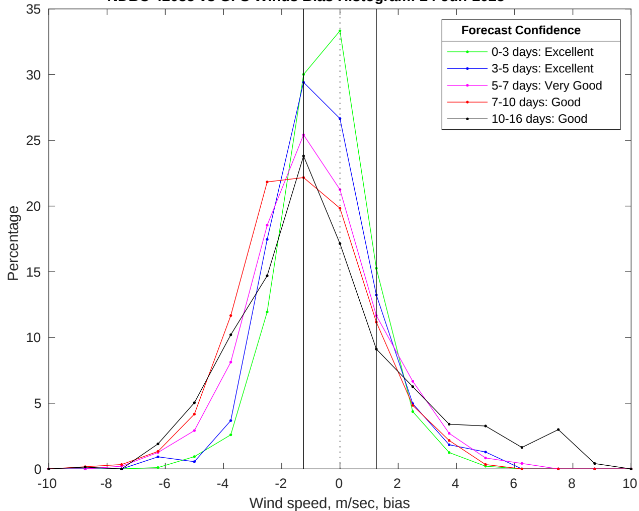
NDBC 42035 vs GFS Winds Bias Histogram: 24-Jun-2025
