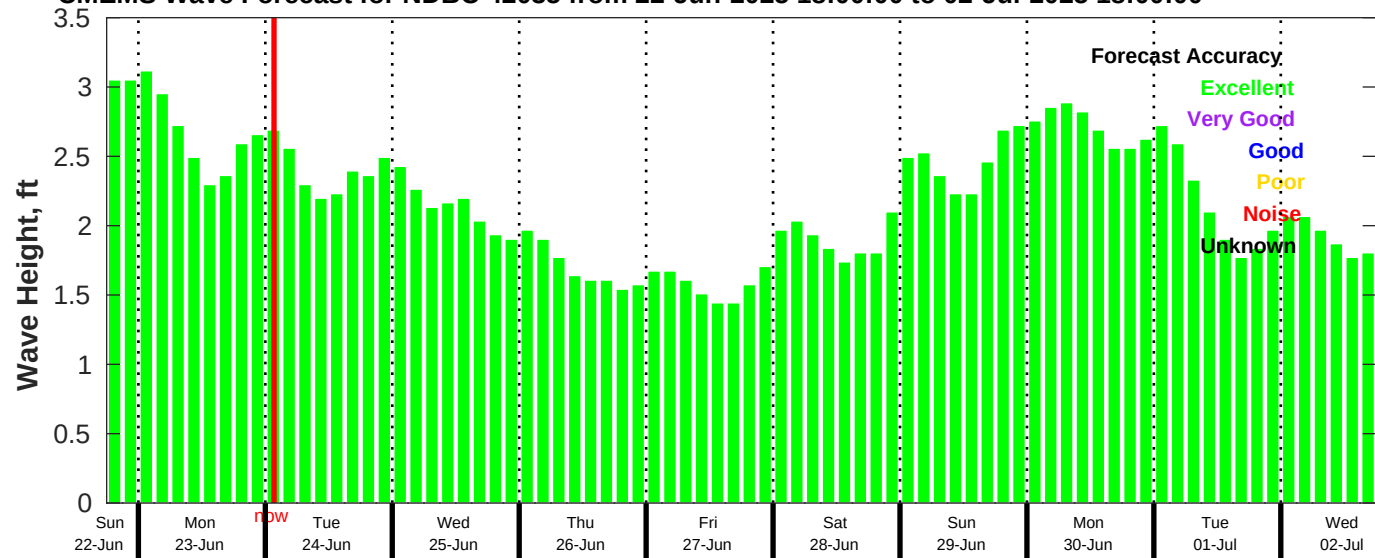
CMEMS Wave Forecast for NDBC 42035 from 22-Jun-2025 18:00:00 to 02-Jul-2025 18:00:00
