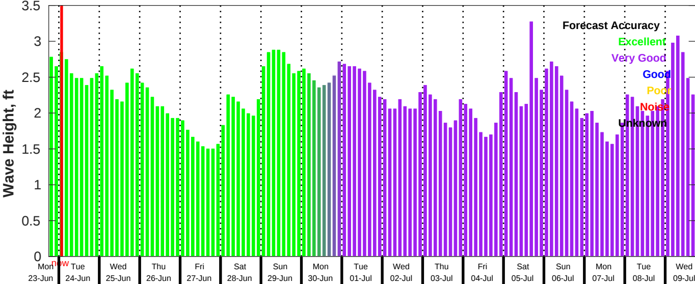
GFS Wave Forecast for NDBC 42035 from 23-Jun-2025 18:00:00 to 09-Jul-2025 18:00:00
