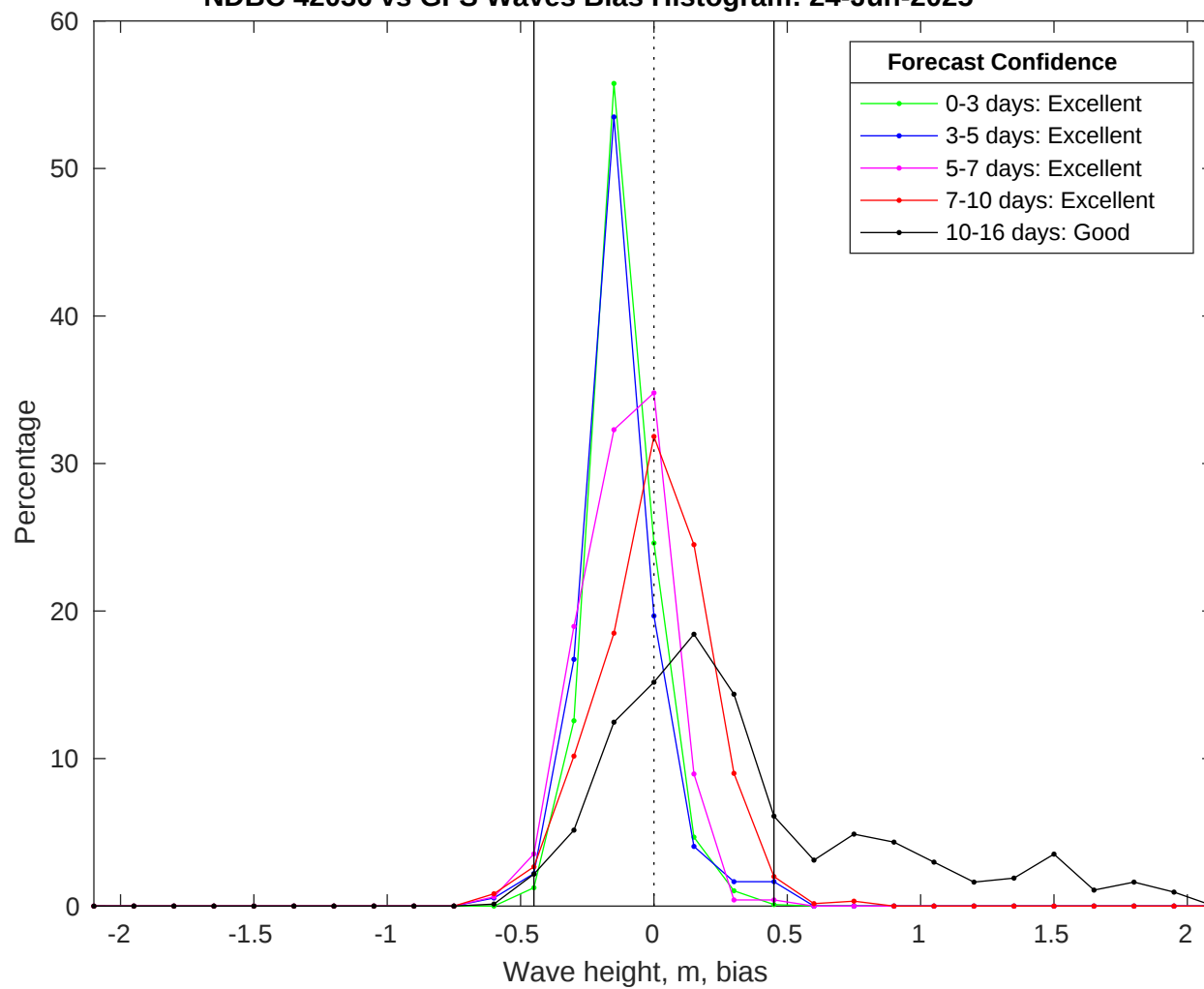
NDBC 42036 vs GFS Waves Bias Histogram: 24-Jun-2025
