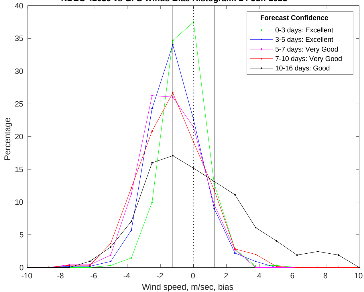
NDBC 42036 vs GFS Winds Bias Histogram: 24-Jun-2025
