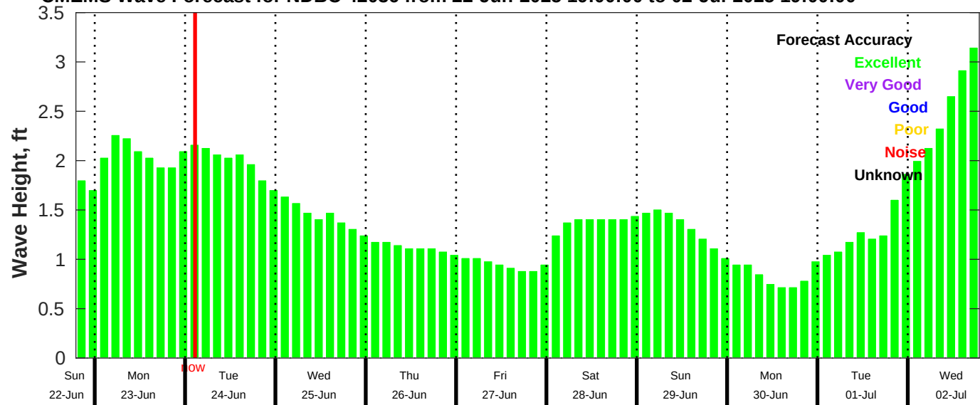
CMEMS Wave Forecast for NDBC 42036 from 22-Jun-2025 19:00:00 to 02-Jul-2025 19:00:00
