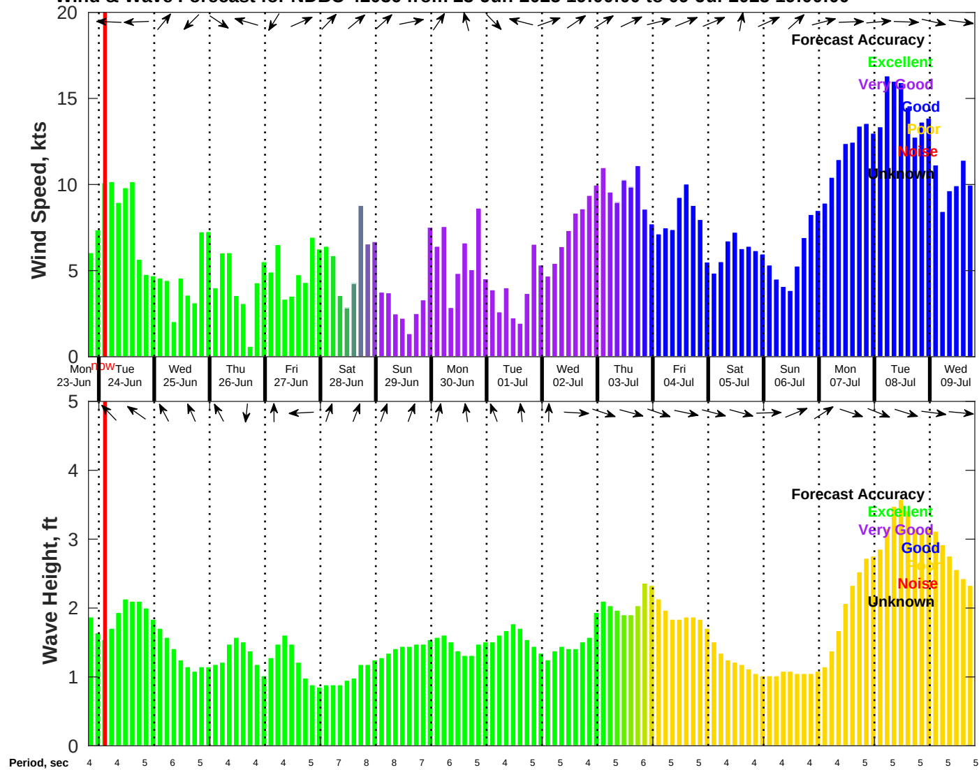
Wind & Wave Forecast for NDBC 42036 from 23-Jun-2025 19:00:00 to 09-Jul-2025 19:00:00
