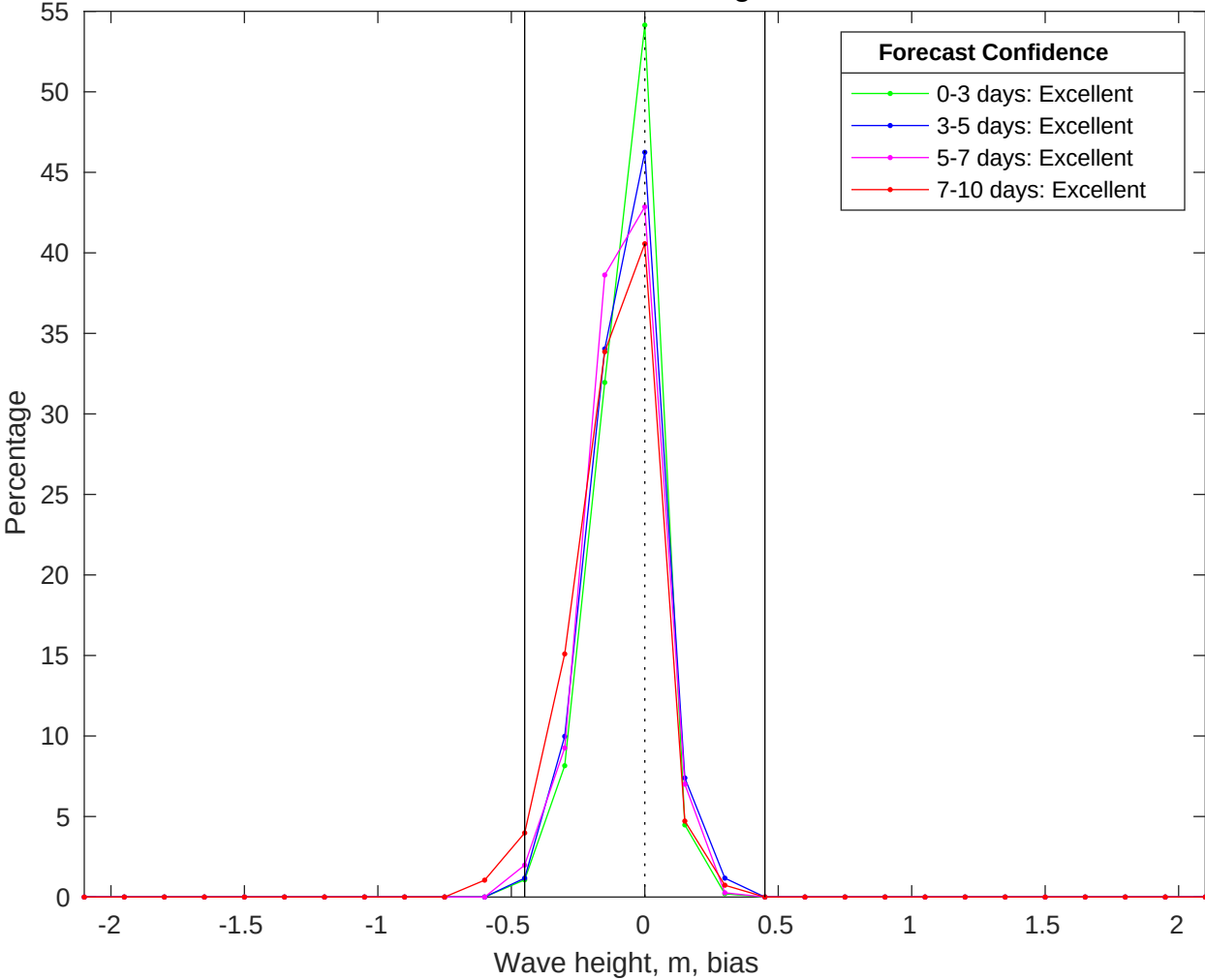
NDBC 42040 vs CMEMS Waves Bias Histogram: 24-Jun-2025
