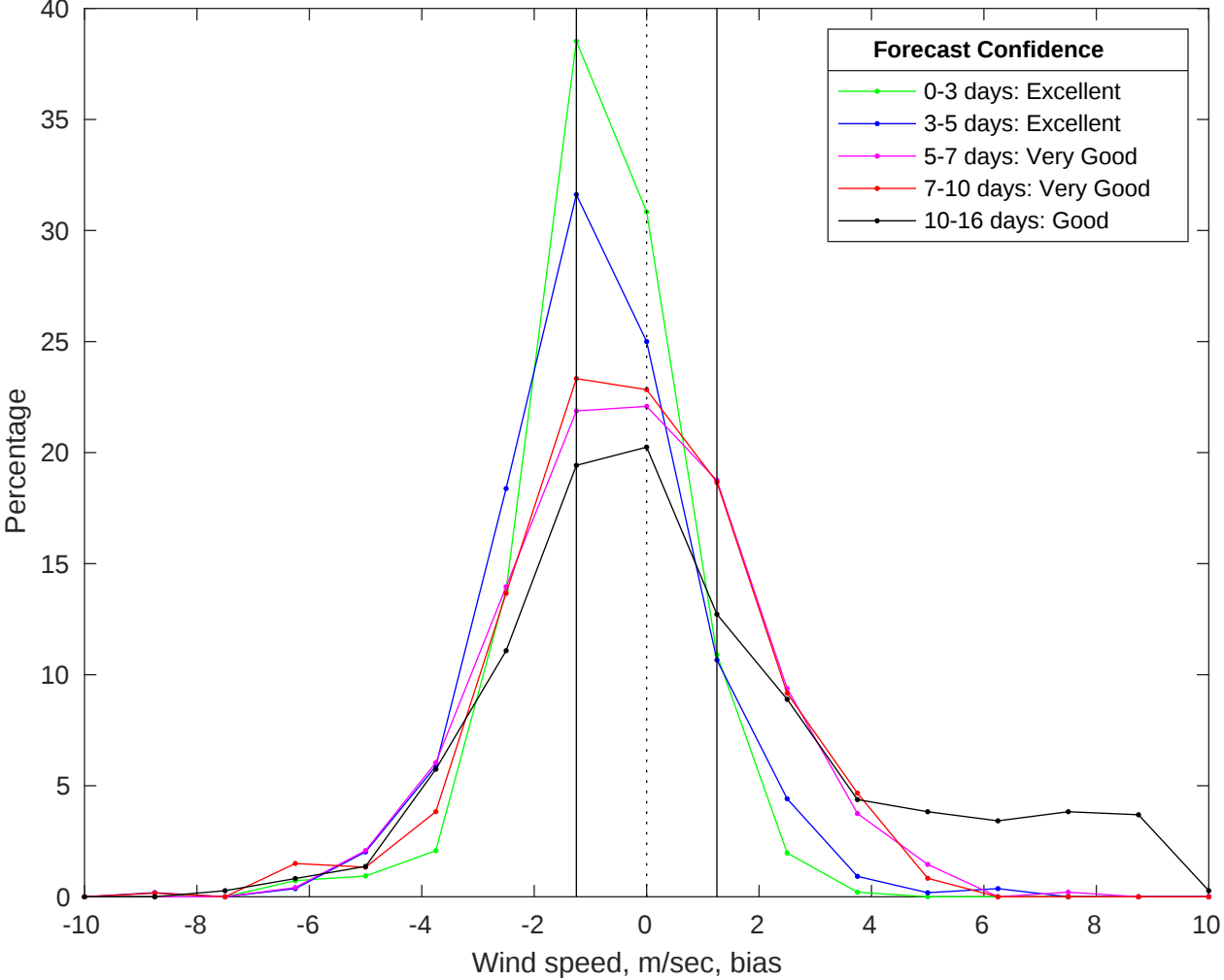
NDBC 42040 vs GFS Winds Bias Histogram: 24-Jun-2025
