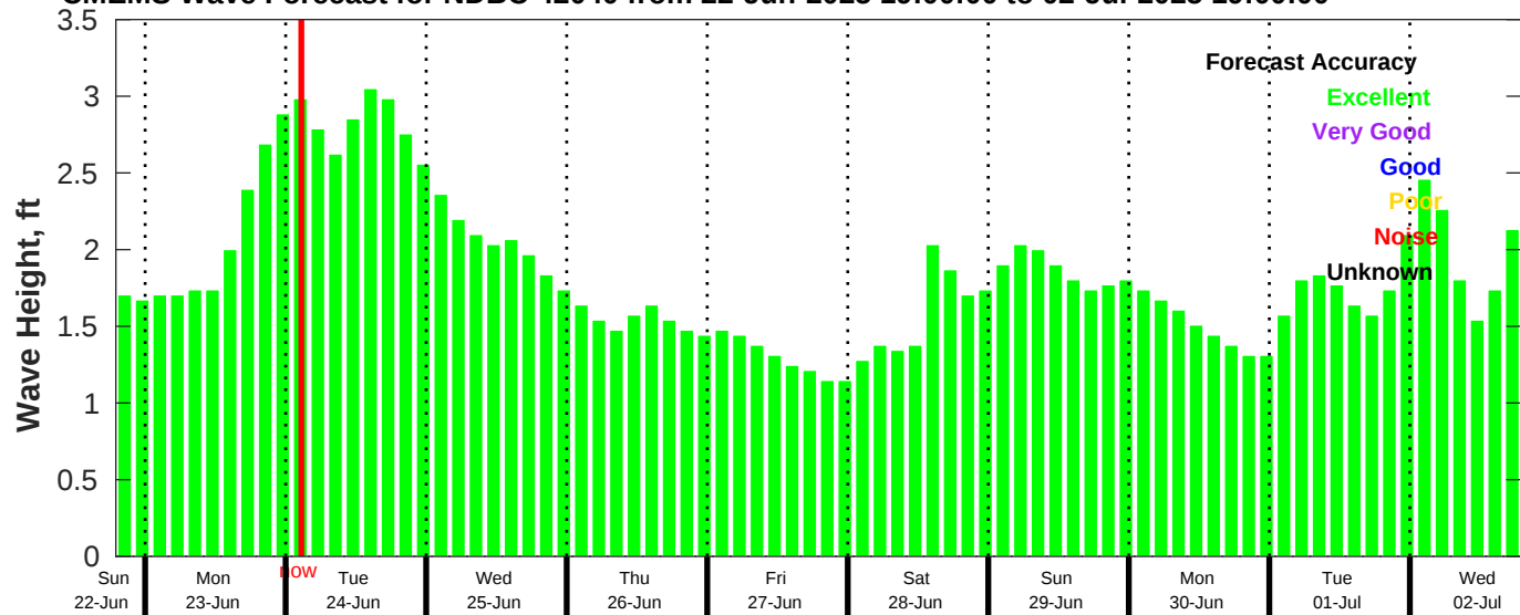
CMEMS Wave Forecast for NDBC 42040 from 22-Jun-2025 19:00:00 to 02-Jul-2025 19:00:00
