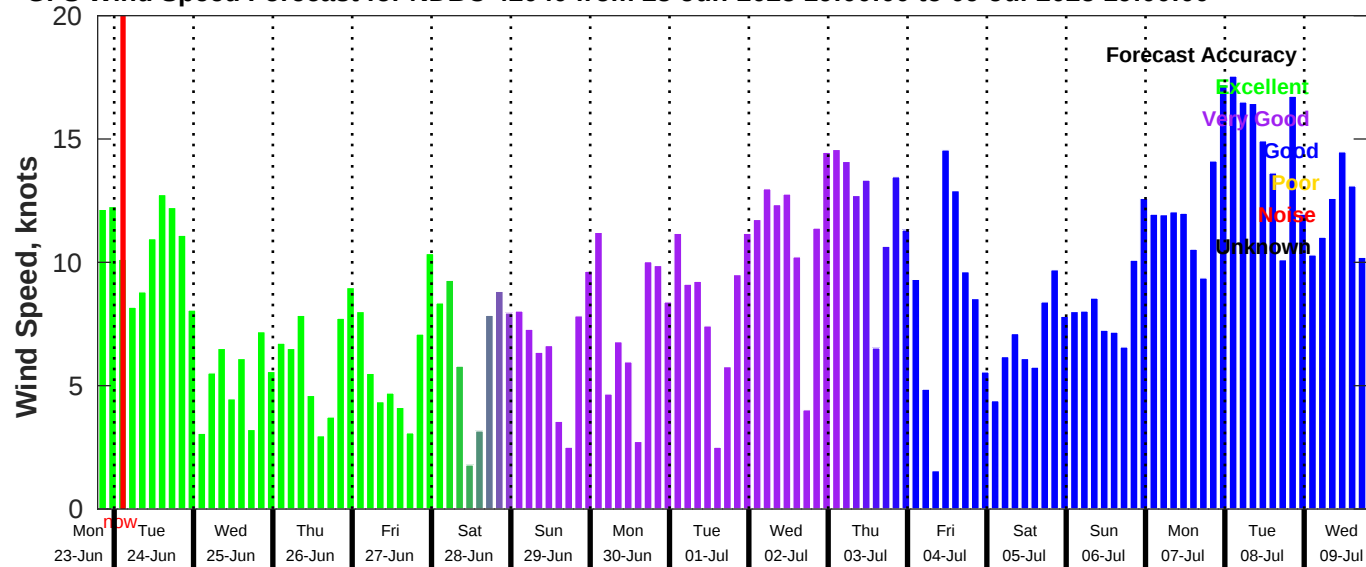
GFS Wind Speed Forecast for NDBC 42040 from 23-Jun-2025 19:00:00 to 09-Jul-2025 19:00:00
