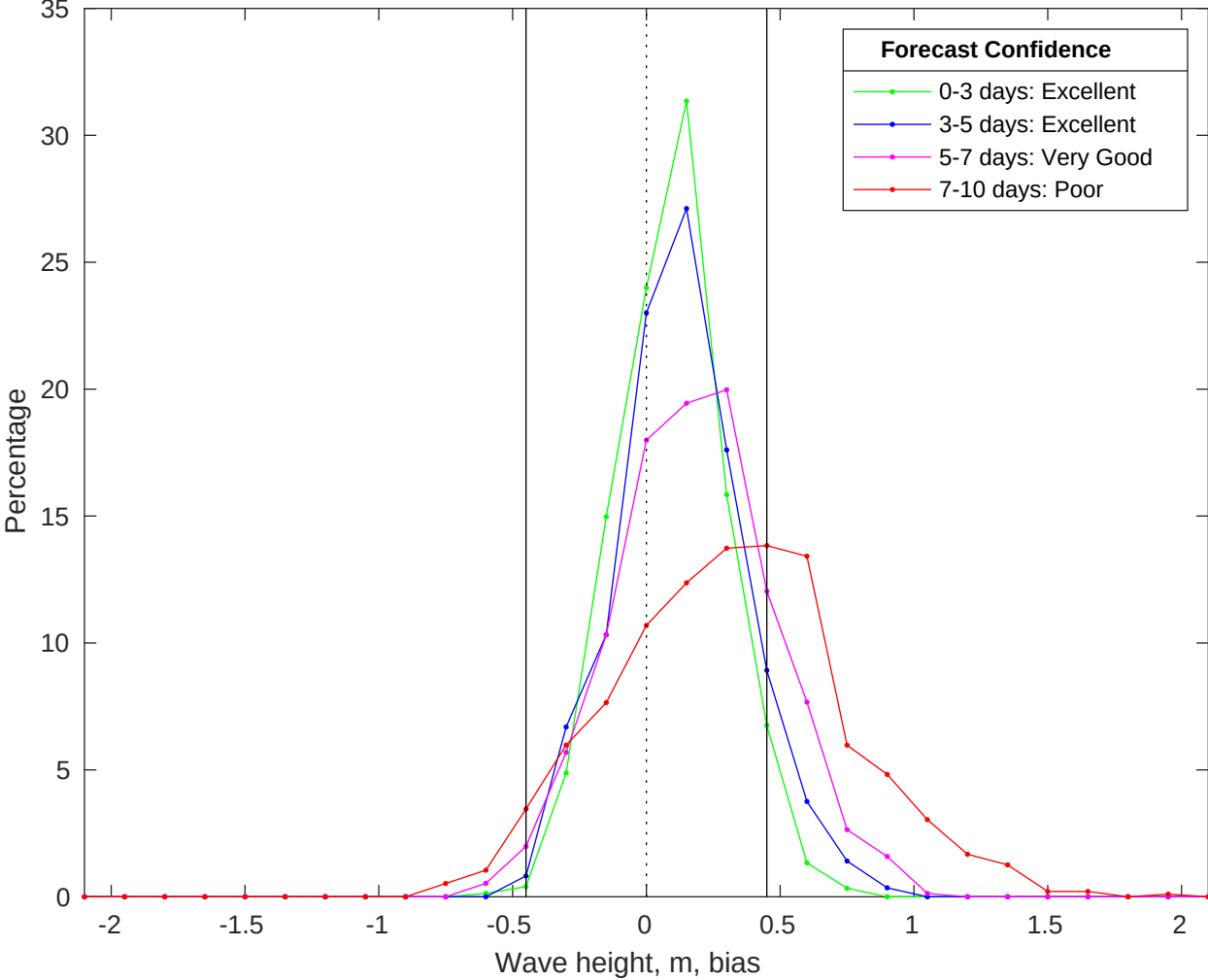
NDBC 46011 vs CMEMS Waves Bias Histogram: 24-Jun-2025
