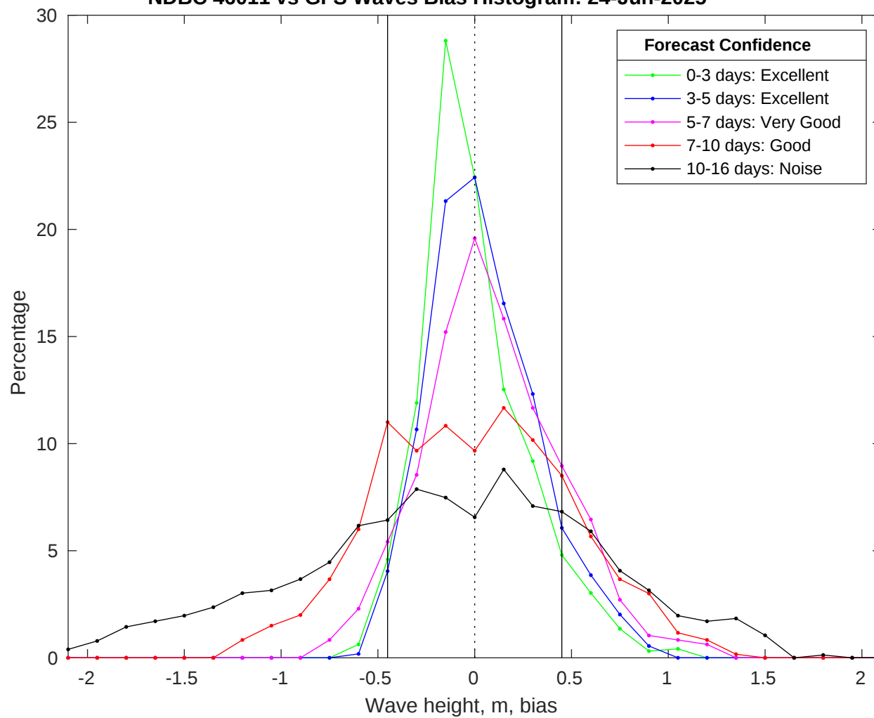
NDBC 46011 vs GFS Waves Bias Histogram: 24-Jun-2025
