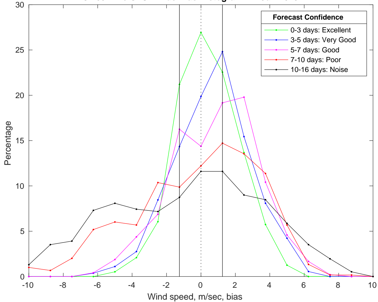
NDBC 46011 vs GFS Winds Bias Histogram: 24-Jun-2025
