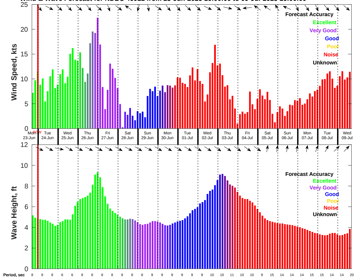
Wind & Wave Forecast for NDBC 46011 from 23-Jun-2025 16:00:00 to 09-Jul-2025 16:00:00
