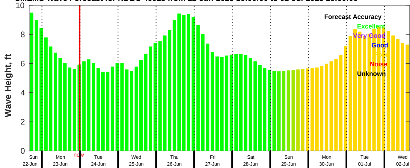
CMEMS Wave Forecast for NDBC 46028 from 22-Jun-2025 16:00:00 to 02-Jul-2025 16:00:00
