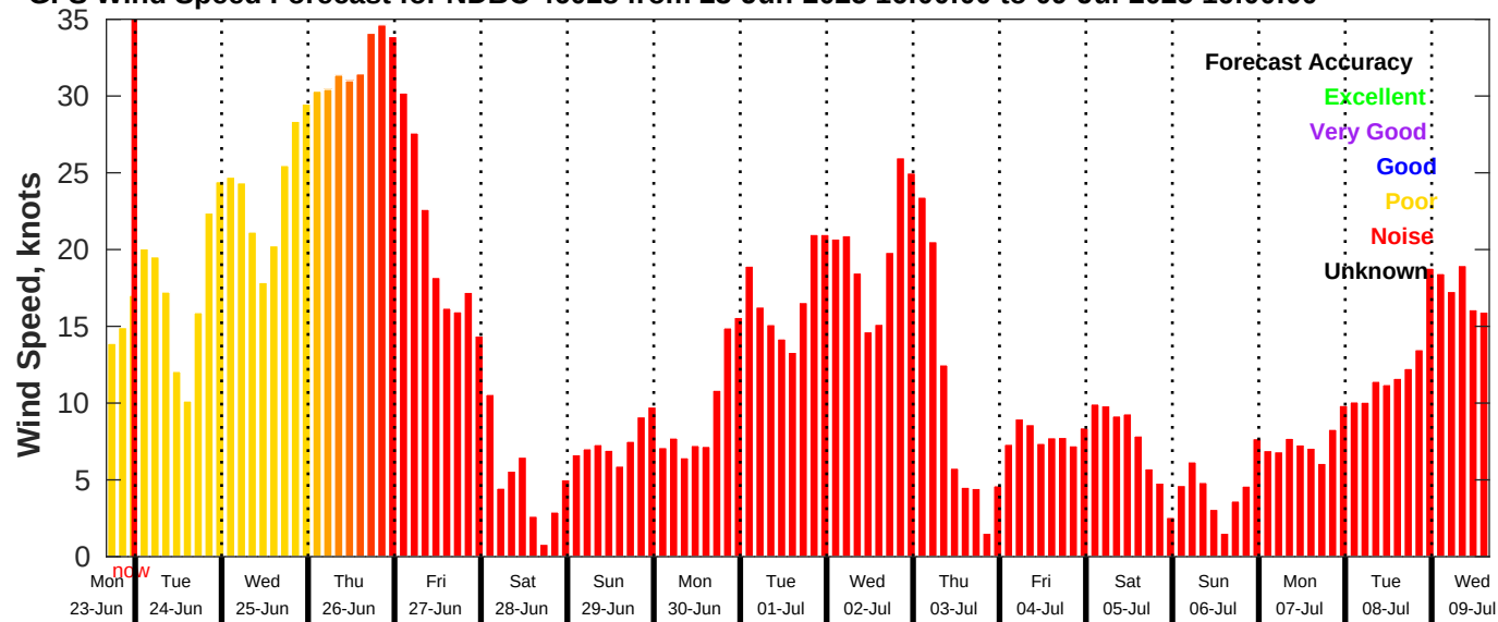
GFS Wind Speed Forecast for NDBC 46028 from 23-Jun-2025 16:00:00 to 09-Jul-2025 16:00:00
