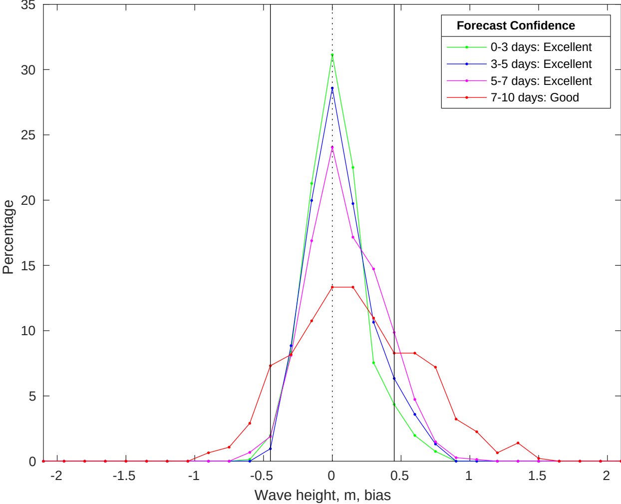
NDBC 46054 vs CMEMS Waves Bias Histogram: 24-Jun-2025
