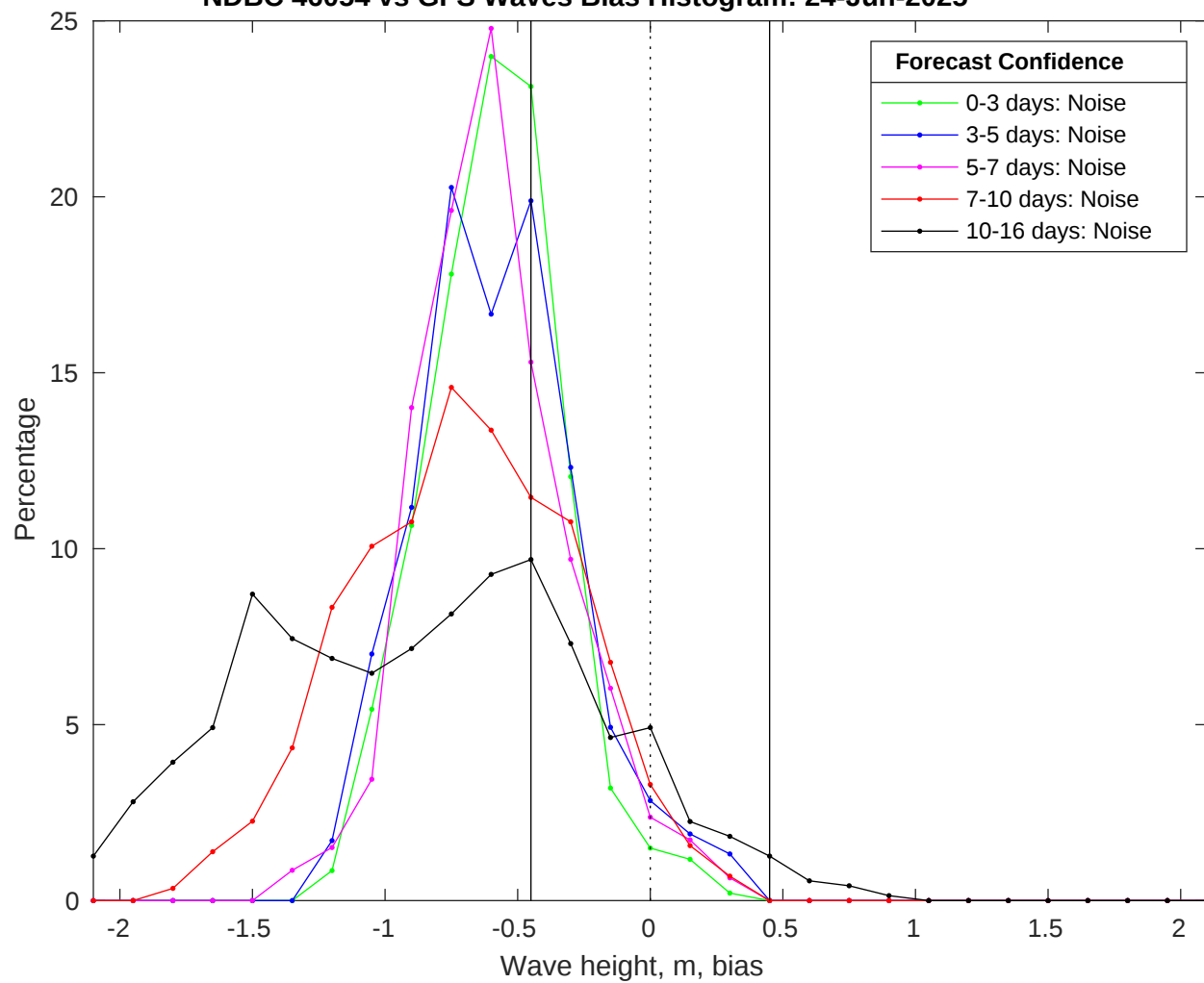
NDBC 46054 vs GFS Waves Bias Histogram: 24-Jun-2025
