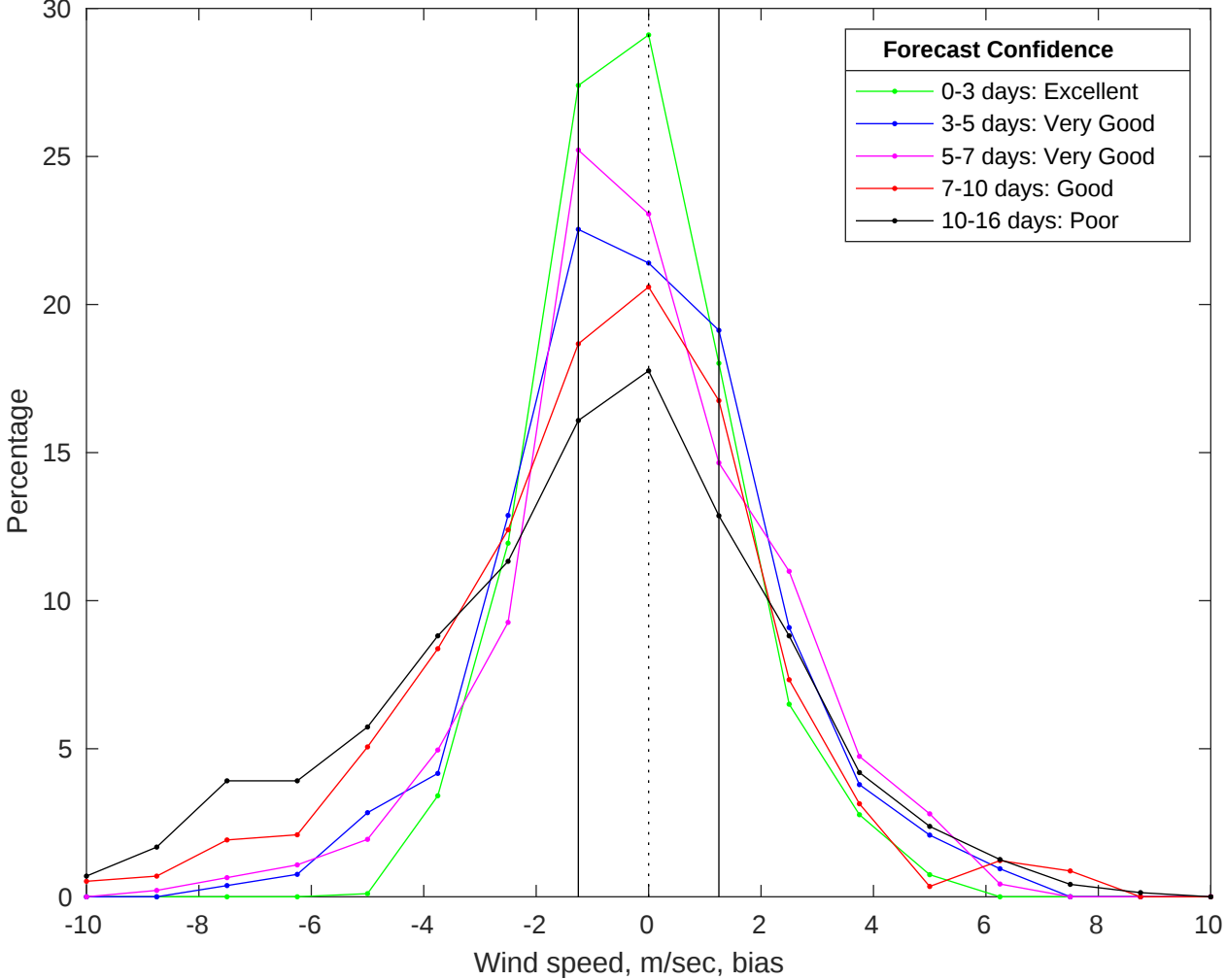
NDBC 46054 vs GFS Winds Bias Histogram: 24-Jun-2025
