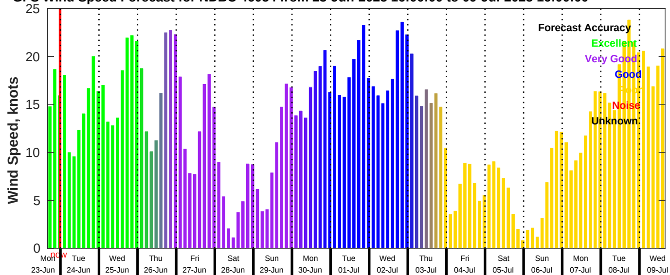
GFS Wind Speed Forecast for NDBC 46054 from 23-Jun-2025 16:00:00 to 09-Jul-2025 16:00:00
